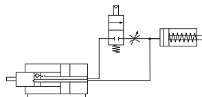
② STOP-Ventil (Blockierventil)
